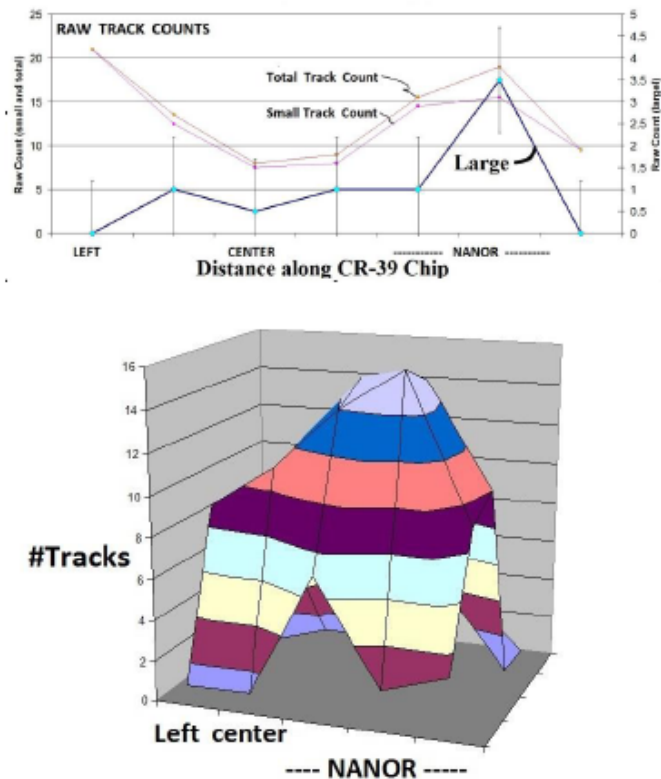
Figure 6. (a) ( top ) The distribution of the density of track counts of small tracks, all tracks, and large tracks as a function of location along a single chip place above the NANOR and the region around it. The NANOR was at the lower left of the flat chip. Importantly, it can be seen that large tracks may be the most useful in imaging CF/LANR systems. (b) ( bottom ) The distribution of density of the large tracks, pixel by pixel, is made over the surface of the CR-39 chip which covered the NANOR and its nearby region, as the NANOR ran continuously over days. Shown is a 3D representation of that large track density count, at this very low resolution pixel number, with the magnitude of the count shown by the height looking up the y-axis. With the same information, Fig. 1 shows the result of rotating this distribution and it shows how it looks directly down that y-axis. Also, confer Fig. 1b which shows the distribution from the vertical axis perpendicular to the long axis of the chip.
