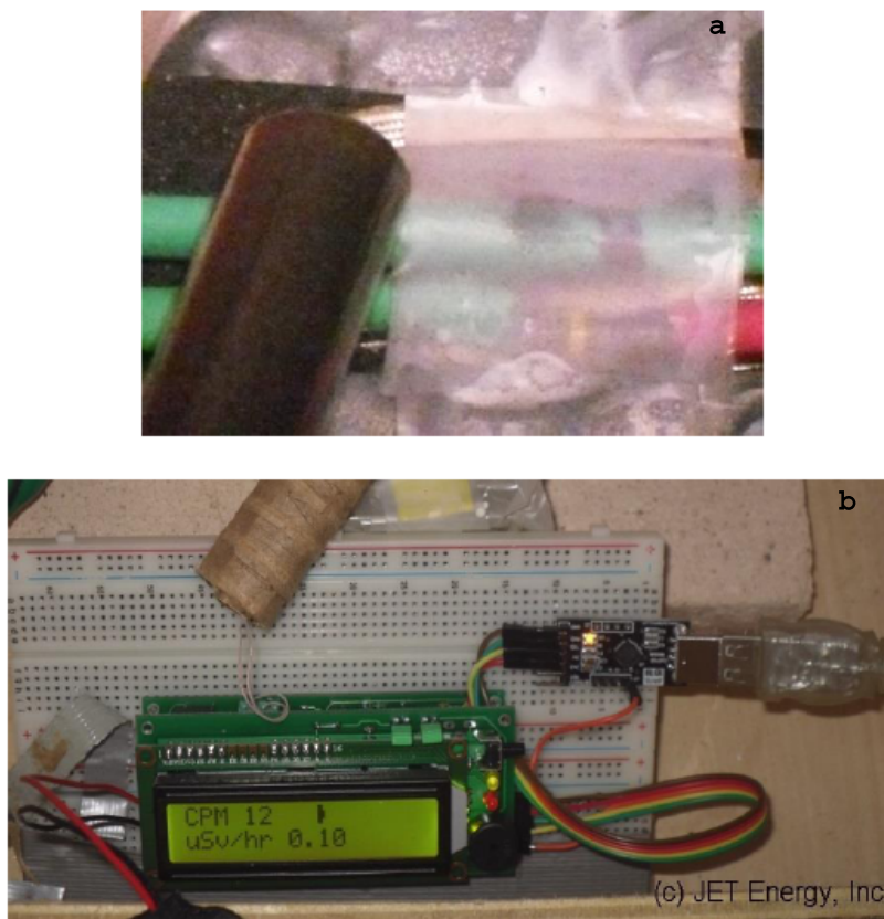
Figure 3. (a) Shown is the central region within the calorimeter. The horizontally directed NANOR-type quantum electronic component, containing active \text{ZrO}_2\text{-PdD} nanostructured material, is located within the upper green cylinder. The Geiger Müller tube is shifted off of the active site (rectangular appearing black area located just above the ohmic resistor (to the right of its yellow-colored band, and off to the right from the center) and shown moved about twice its width to the left from its normal location for the photograph. The Geiger–Müller tube is just outside of the tape and to left for the photograph. In addition, the holders, thermal ballasts, thermal conduction materials, vicinal detectors, and electrical insulation, have been removed to more clearly show this. (b) The modified Arduino delivered 500–700 V to the GM tube while also recording GM output, integrating that to CPM, and a 10 min running average of CPM, and converting to microSv/h. The output was delivering (including tube voltage) to the USB to the second DAQ, and to a charlieplexed digital output over the Arduino (shown with background levels).
