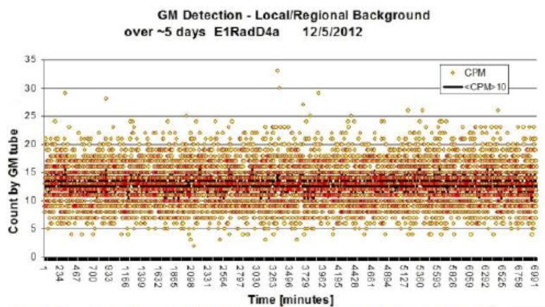
Figure 4. A five-day collection of background data. Shown is the 10 min moving average of the CPM, \langle \text{CPM} \rangle_{10} , as a function of time (Fig. 5). For this long measurement, the LANR NANOR, the ohmic control, and the electrical driving system was in place but remained electrically off, for the entire time.
