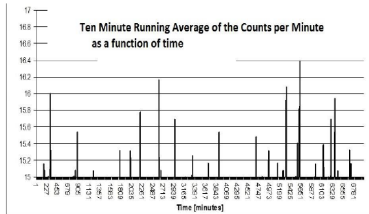
Figure 5. A five-day collection of “high-pass” background data. Shown is \langle\text{CPM}\rangle_{10} , as a function of time, but only shown are those events which exceeded \langle\text{CPM}\rangle_{10} greater than 15. In the following, a high pass filter was used which only “passes” the \langle\text{CPM}\rangle_{10} which are greater than \sim 15.5 .
