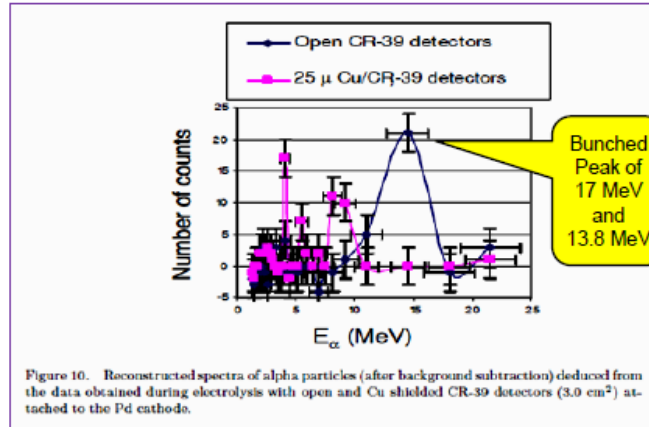
Observation of alpha-particles with CR39 detector by A. Lipson et al, ICCF10
