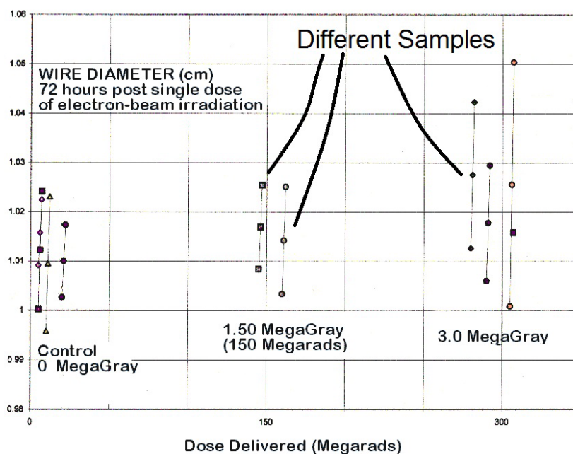
Figure 3. Palladium wire diameter three days after electron-beam irradiation-created vacancy states.
