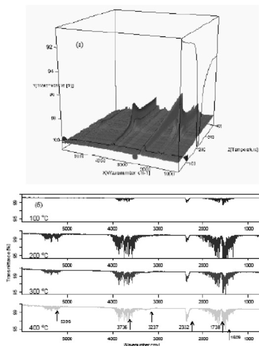
Figure 2. IR absorption for interboride .
