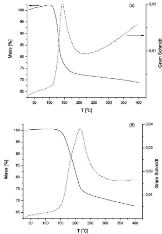
Figure 1. TGA (Thermo-gravimetric analysis) analysis for interboride (top) and ulexite (bottom).
