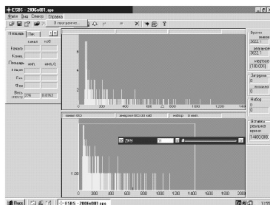
Figure 5. Calibration spectrum of alpha-particles source with the use of isotope \text{Pu}^{239} .
