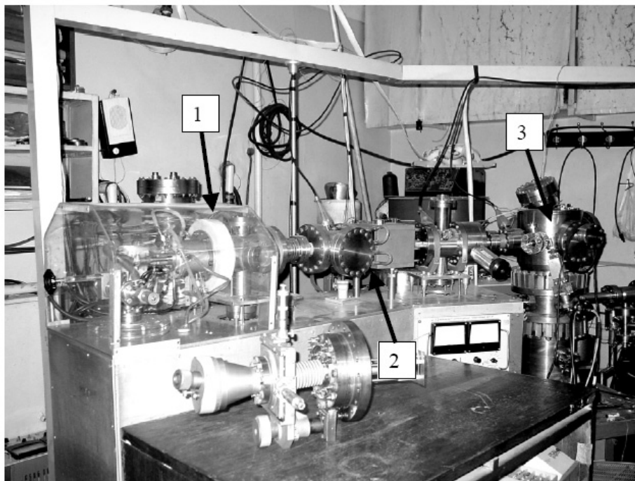
Figure 1. A general view of experimental installation.
