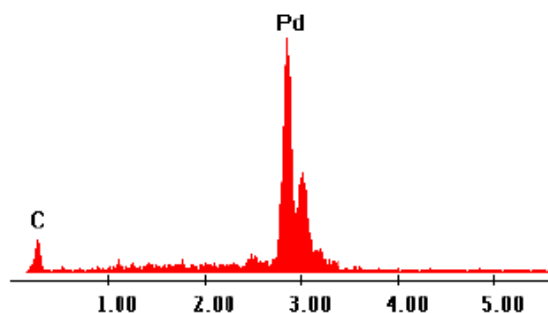
Figure 8. EDS of Pd origin sample before triggering.
