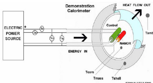
Figure 2. Electric driver and calorimeter showing parallel diagnostics consisting of heat flow measurement and temperature, and the ohmic (thermal) control. The electric power supply provided a high voltage DC rail voltage with the electronics controlling the applied voltage across the component.
