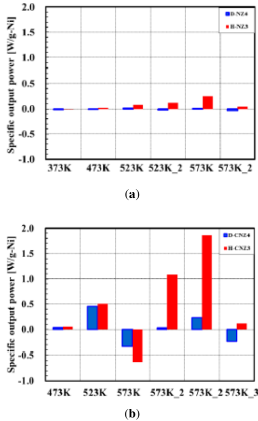
Figure 12. Specific output power data for the s-phase of sample H(D)–NZ, upper figure (a) and H(D)–CNZ, lower figure (b).
