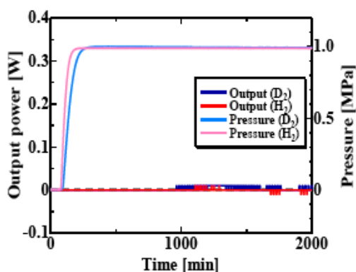
Figure 5. Results of \text{D}_2/\text{H}_2 absorption runs for Ni–Zr oxide compounds; the run numbers are D–NZ1#1 and H–NZ2#1.
