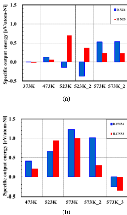
Figure 13. Specific output energy data for the t-phase of sample H(D)–NZ, upper figure (a) and H(D)–CNZ, lower figure (b).
