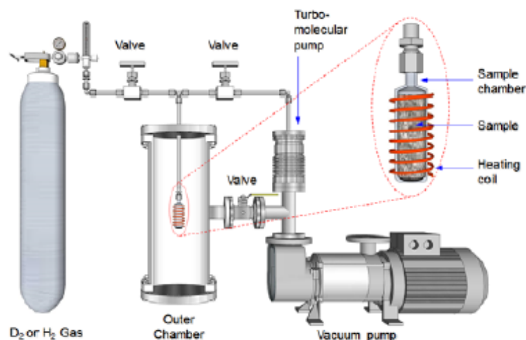
Figure 3. Sketch of the gas-loading system.
