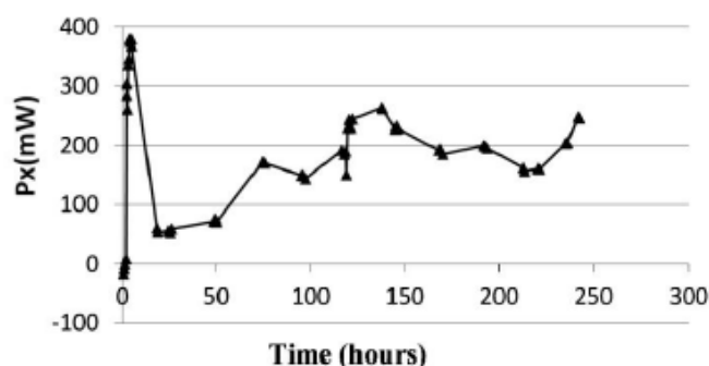
Figure 2. Calorimetric results for the co-deposition of palladium in \text{D}_2\text{O} at 300 mA.
