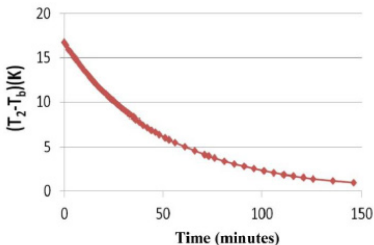
Figure 4. Experimental cooling curve for the Pd/H 2 O experiment.
