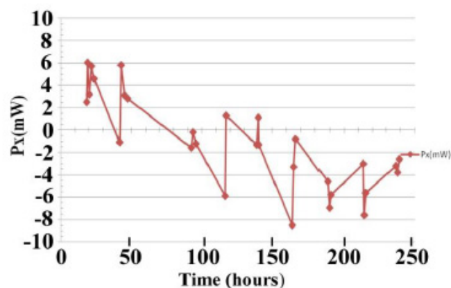
Figure 1. Calorimetric results for rhenium co-deposition in \text{H}_2\text{O} (thermistor 4).
