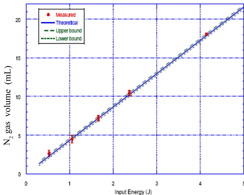
Figure 2. Wide range calibration of the cryogenic calorimeter with a 10 \Omega resistor. Error range is \pm 0.06 J.
