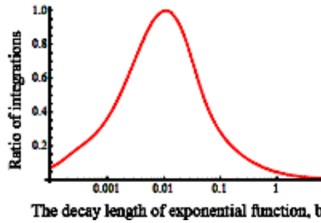
Figure 3. Qualitatively showing the maximum of overlapping was reached when binding energy of n + {}^{58}\text{Ni} is of order of MeV.
