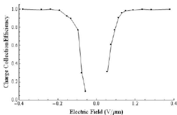
Figure 4. Charge collection efficiency versus applied bias across the diamond sensor during Pu-239 exposures.
