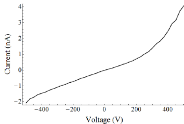
Figure 2. I – V characteristics of the diamond sensor.
