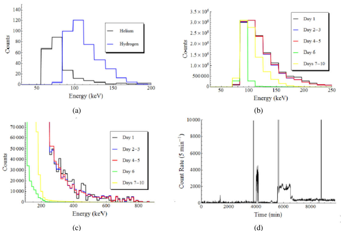
Figure 6. Experimental results obtained in the gas loading palladium electrode on a diamond sensor. Here the results are shown for (a) the background spectra obtained for hydrogen and helium, (b) and (c) the low-energy spectra from the deuterium run, and (d) the count rate of pulses observed in the diamond sensor over time for the deuterium run.
