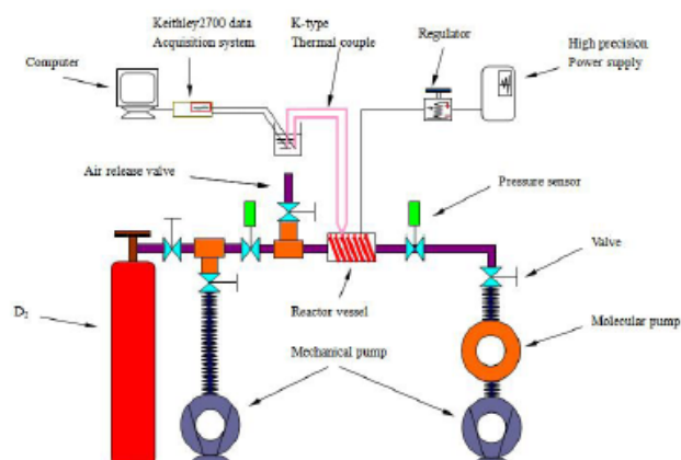
Figure 1. Deuterium gas loading palladium film system.
