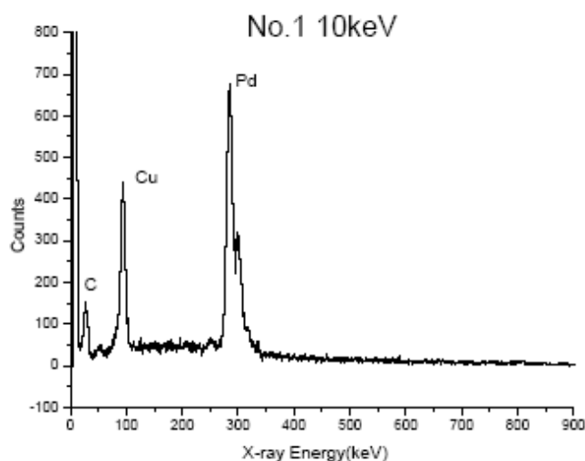
Figure 11. No. 1 sample 10 keV EDS.
