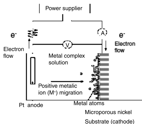
Figure 1. Electrolytic co-deposition cells.
