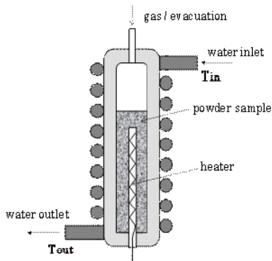
Figure 1. Schematic of the calorimeter.
