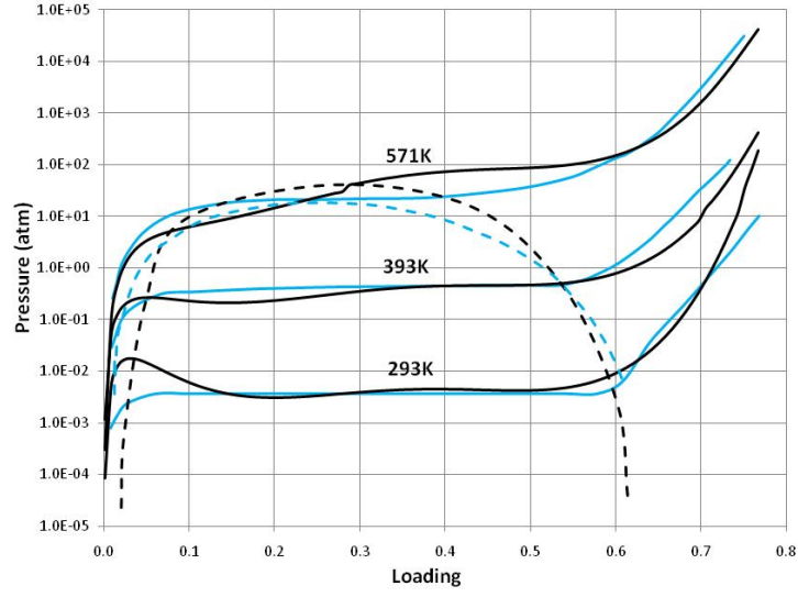
Figure 3. P–C–T isotherms; model (black); experiment (blue).
