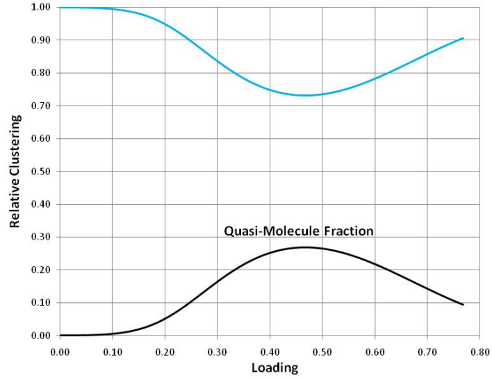
Figure 9. Quasi-molecule fraction from optimization of the model.
