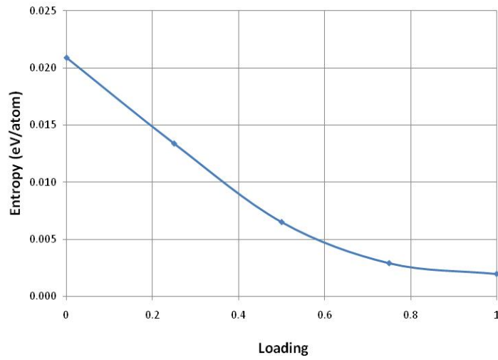
Figure 7. Model electronic entropy at 571 K.
