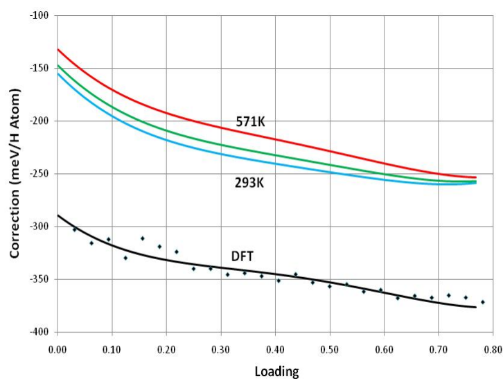
Figure 14. Interaction energy corrections for the pairing model.
