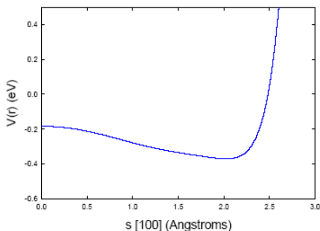
Figure 9. Model H 2 or D 2 potential in as a function of distance in the [100] direction of a monovacancy with seven interstitials.
