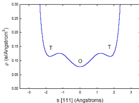
Figure 2. Background electron density along the [111] for Pd (with a = 4.081 Å).
