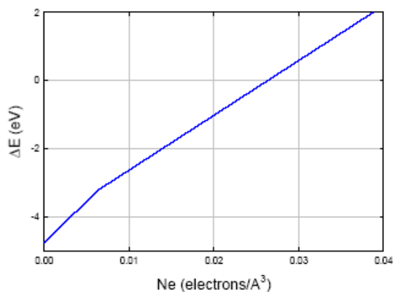
Figure 5. Embedding energy for H_2 with vacuum separation [12].
