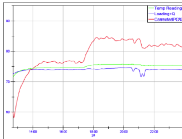
Figure 6. Plot of power gain (%), temperature ( ^{\circ}\text{C} ), and proprietary pulse parameter (blue) versus time of day for Experiment 4.
