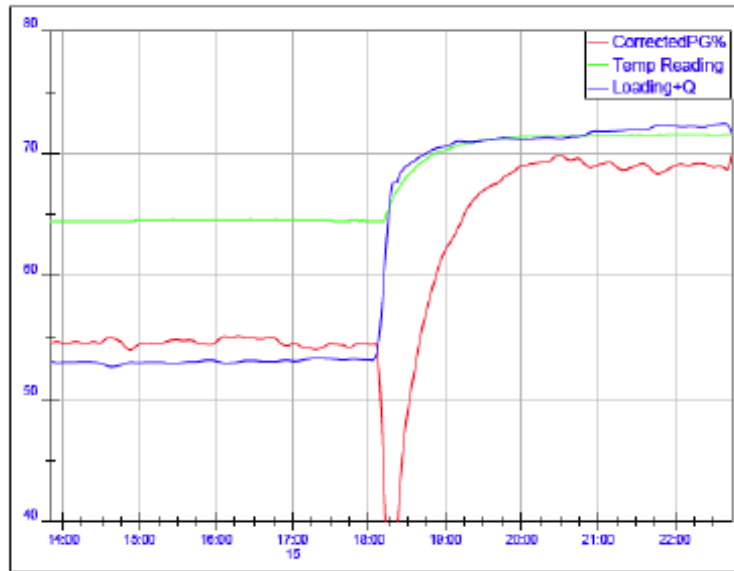
Figure 5. Plot of power gain (%), temperature ( ^{\circ}\text{C} ), and proprietary pulse parameter (blue) versus time of day for Experiment 3 continued.
