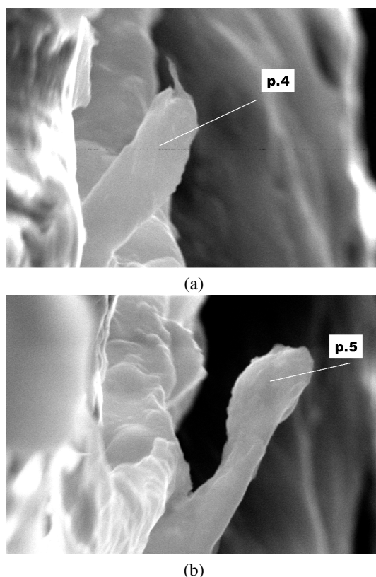
Figure 4. Two congealed blowouts from the direction of \gamma -quanta escape from the right end of the palladium wire.
