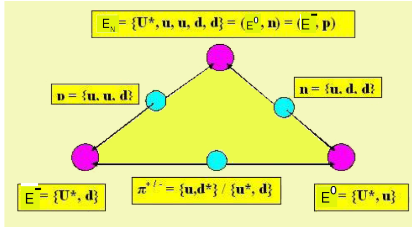
Figure 1. The Erzions and Enion structural quark scheme.
