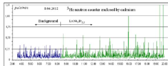
Figure 9. Count rate of ^3\text{He} neutron counter, wrapped up in cadmium sheet. Arrangement under cadmium of \text{LaNi}_5 sample, loaded by deuterium, increases significantly of bursts frequency and amplitude.
