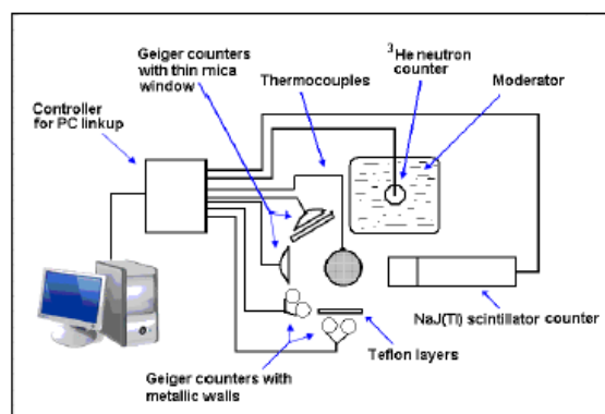
Figure 2. Equipment complex for radiation and thermal measurements.
