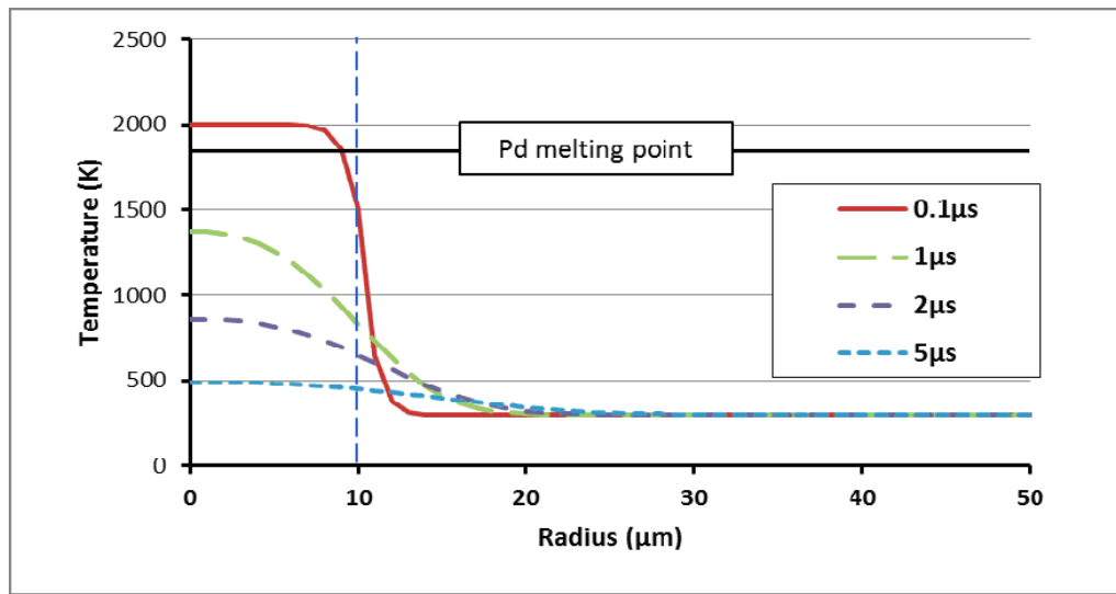
Figure 11. Evolution of the temperature for a 20 \mu\text{m} diameter core – Assumed reaction time is 0.1 \mu\text{s} .
