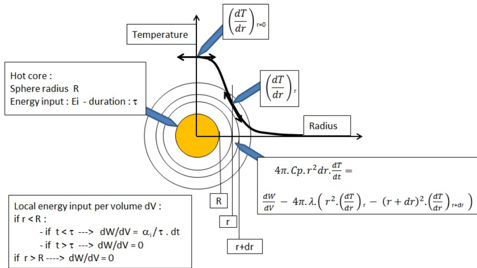
Figure 8. Schematic representation of the heat flow model.
