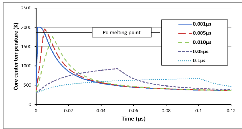
Figure 10. Evolution of the temperature at the centre of a 2 \mu\text{m} core – Influence of the reaction time.
