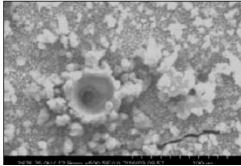
Figure 1. Large crater with a rounded shape. There are evident signs of melting of the ejected material, some of it solidified around the crater rim. The diameter is 50 \mu\text{m} . The original point of the explosion seems to be located several tens of \mu\text{m} below the surface [3].
