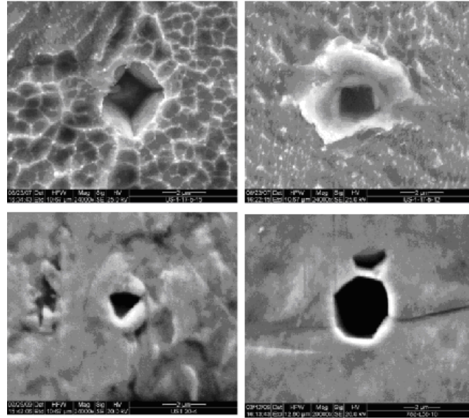
Figure 4. Micrographs of small craters from Super-wave experiments by M. Tsirlin . Published by Nagel [6]. The diameters range from 1 \mu\text{m} to 2 \mu\text{m} . There are no signs of melting. The shapes appear to be influenced by the cathode crystal structure.
