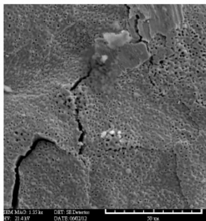
Figure 9. Detailed SEM examination of the Pd–Ni surface after the study.
