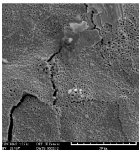
Figure 8. SEM image of a surface of Ni on Pd after the study containing voids and cracks.
