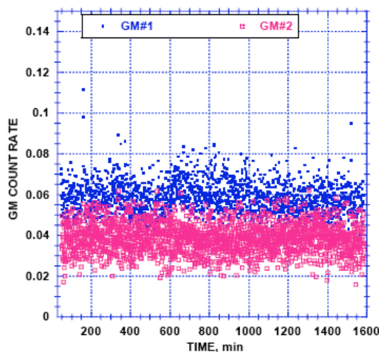
Figure 19. Behavior of GM No. 1 and GM No. 2 when a typical inert sample is in the apparatus. The difference between the two GM count rates is arbitrary. Only the constant value over time is important.
