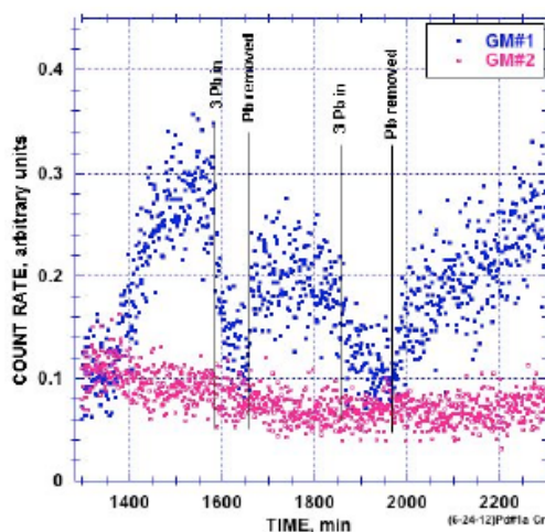
Figure 12. Sample of Pd coated by Cr. Time sequence taken from Fig. 12.
