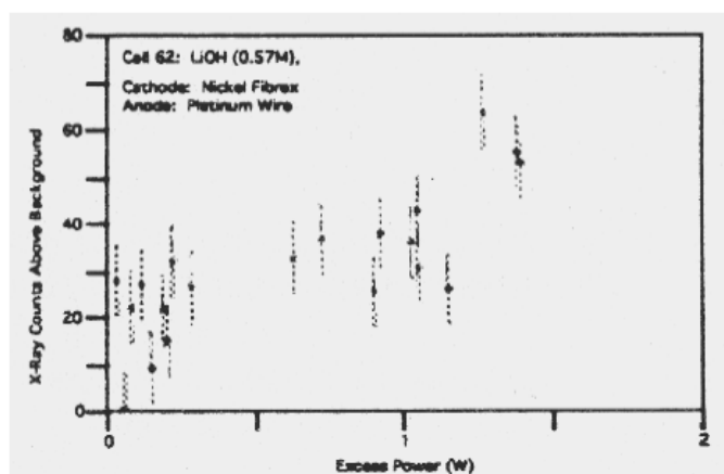
Figure 4. Radiation detected by Bush and Eagleton [17] from a cell having a Ni cathode and \text{H}_2\text{O} electrolyte while it was making excess power.
