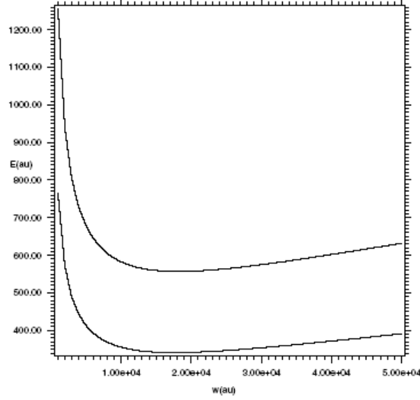
Figure 2. Energy versus variational parameter, w , for two Landau-type states of the Dirac equation for b = a^2 . Upper: a = 0.19 . Lower: a = 0.565 . The binding energy is mc^2 - E .
