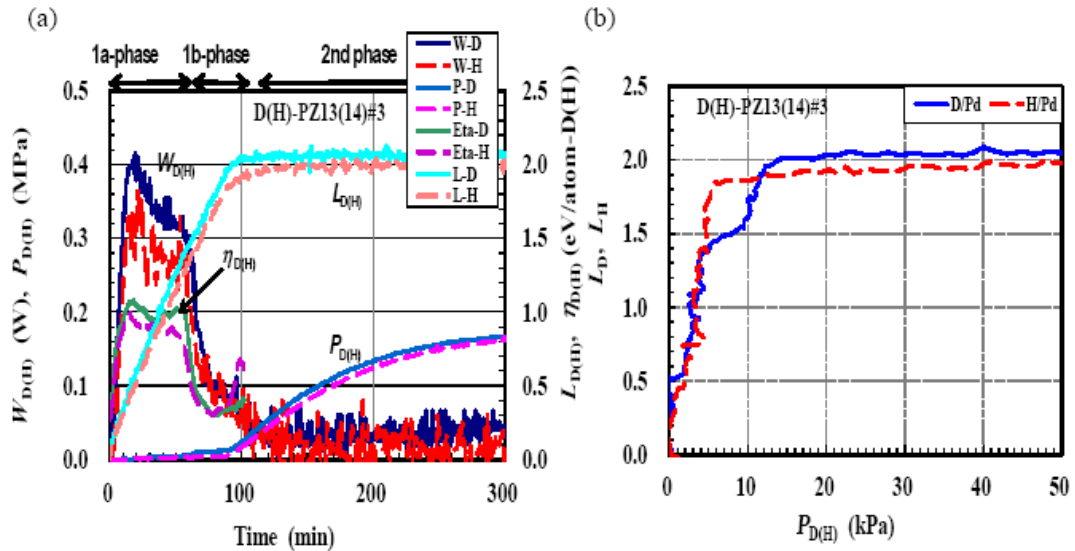
Figure 3. (a) Typical traces of output power W(t) , pressure P(t) , time-resolved loading ratio L(t) and time-resolved specific sorption energy \eta(t) , (b) L(t) – P(t) diagram of the PZ13(14)# 3 runs.
