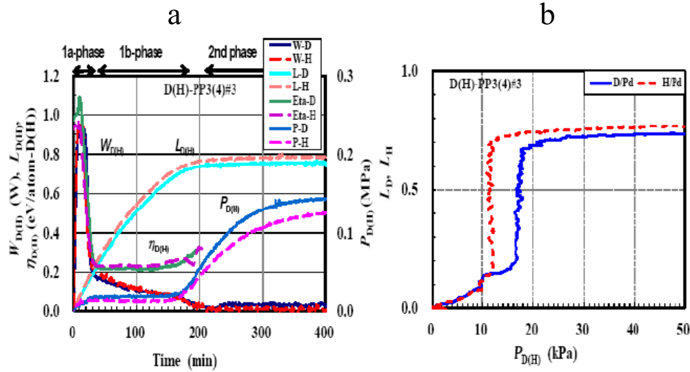
Figure 5. (a) Output power W(t) , pressure P(t) , time-resolved loading ratio L(t) and time-resolved specific sorption energy \eta(t) , (b) L(t) - P(t) diagram of the PP3(4)#3 runs.
