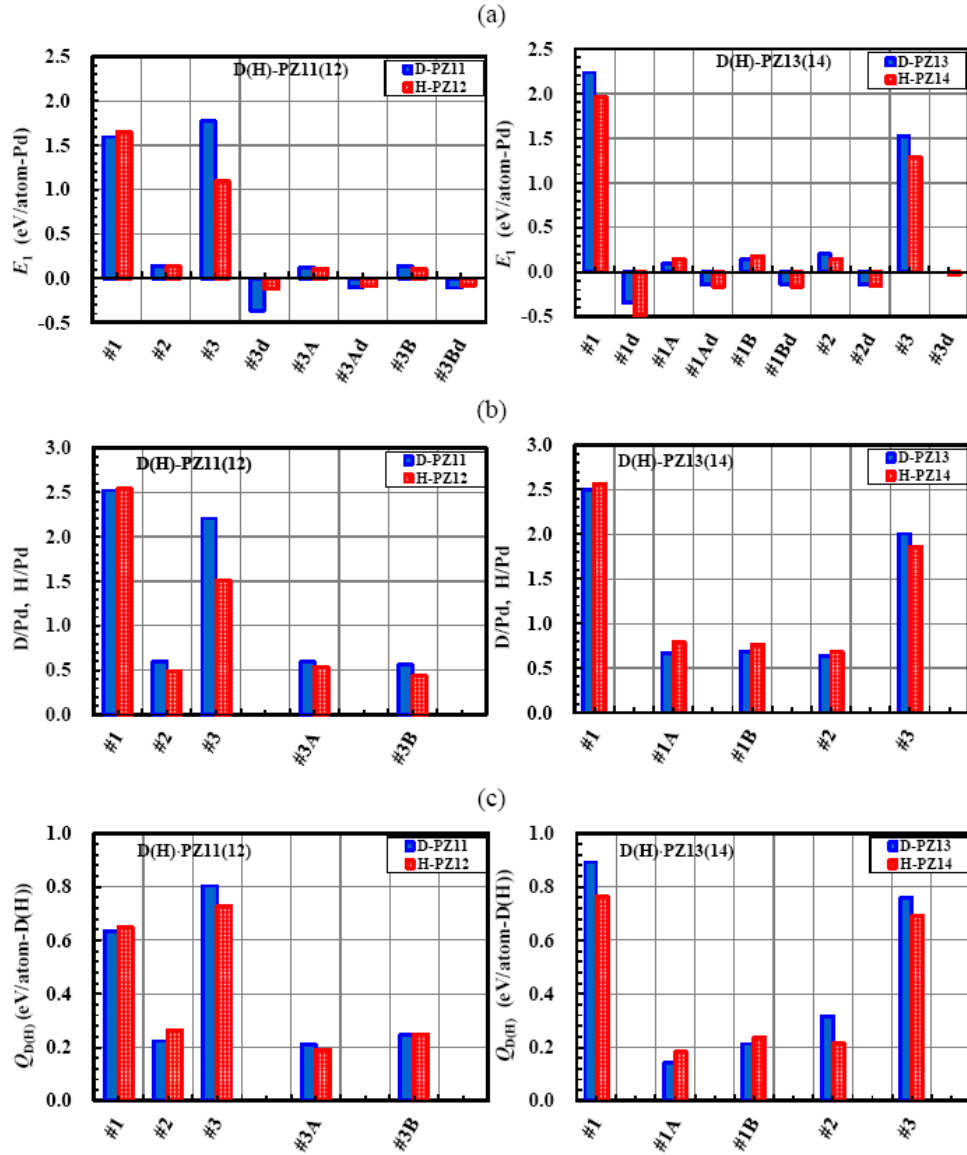
Figure 4. First-phase absorption parameters of the PZ sample; (a) first-phase specific output energy, E_1 , (b) the loading ratio, D(H)/Pd, and (c) the hydridation energy, Q_{D(H)} .
