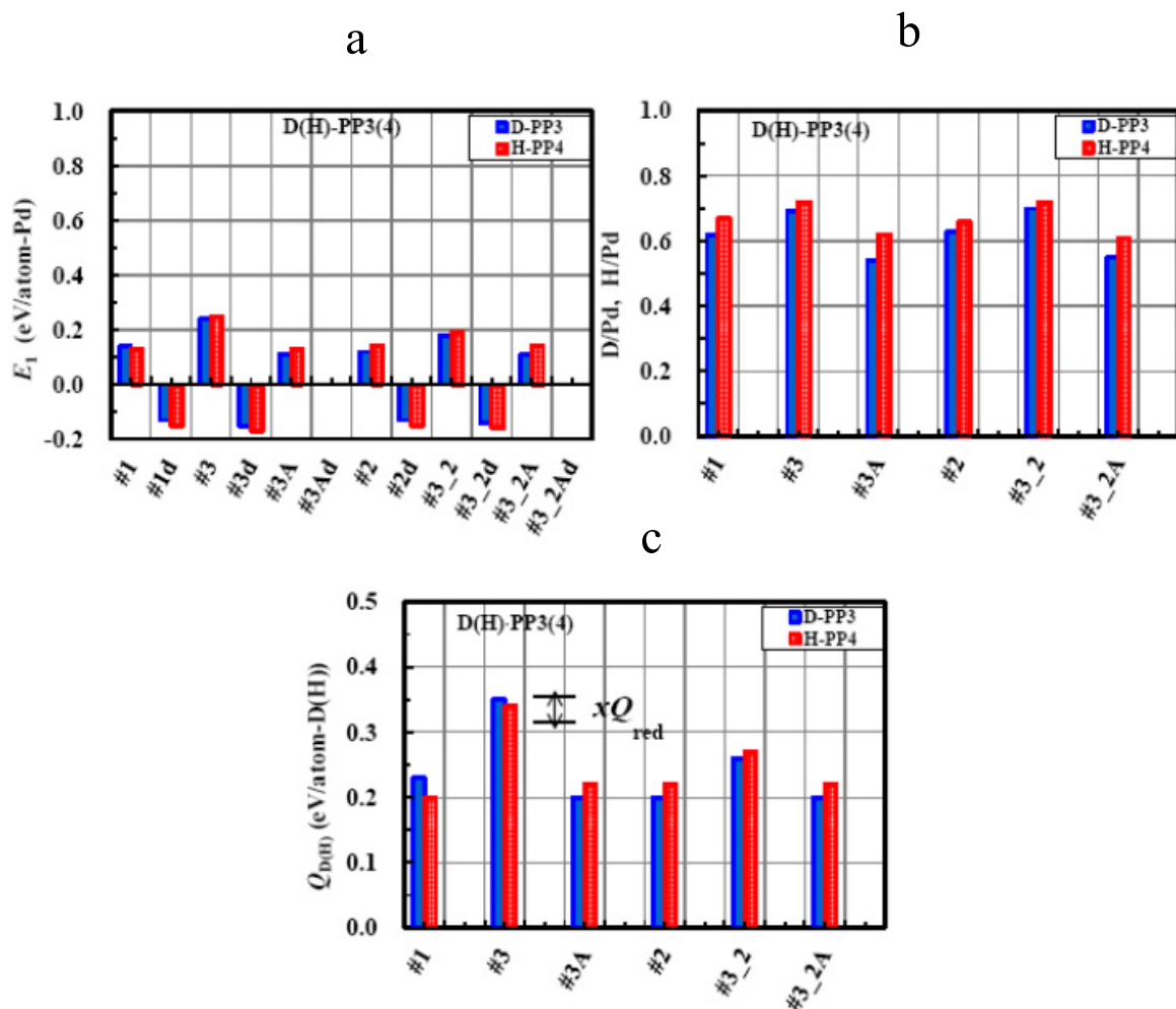
Figure 6. First-phase parameters of the D-PP3#3 and the H-PP4#3 runs.
