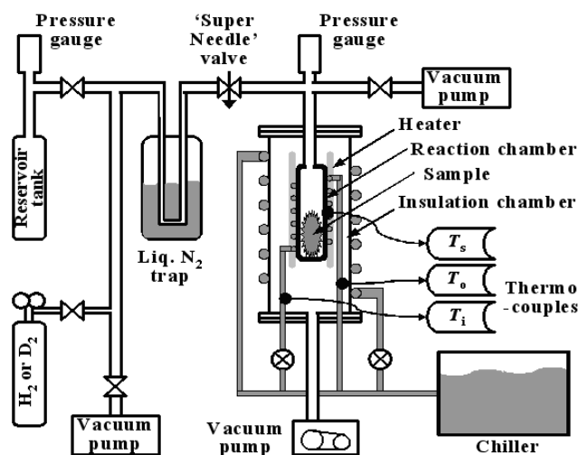
Figure 1. Schematic of one part of the twin system.
