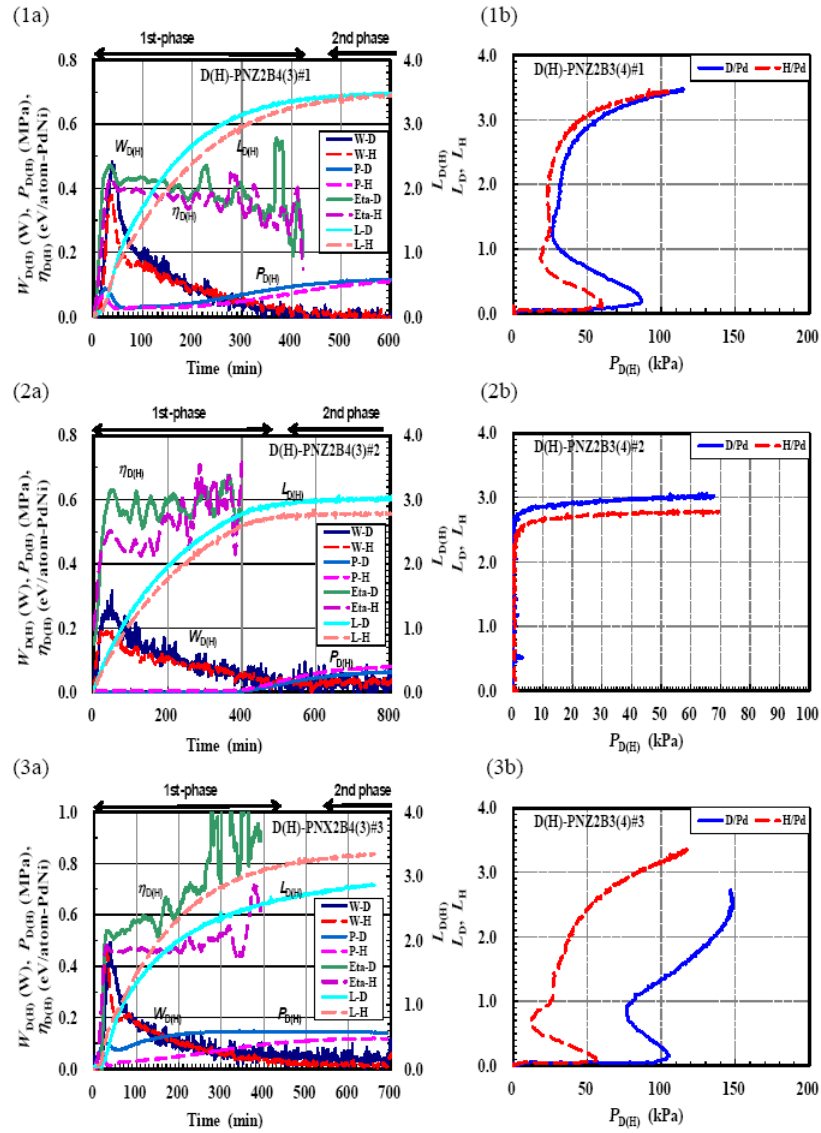
Figure 9. (1a,2a,3a) Output power W(t) , pressure P(t) , time-resolved loading ratio L(t) and time-resolved specific sorption energy \eta(t) , (1b,2b,3b) L(t)-P(t) diagram of the H(D)-PNZ2B3(??)#1, H(D)-PNZ2B3(??)#2 and H(D)-PNZ2B3(??)#3 runs.
