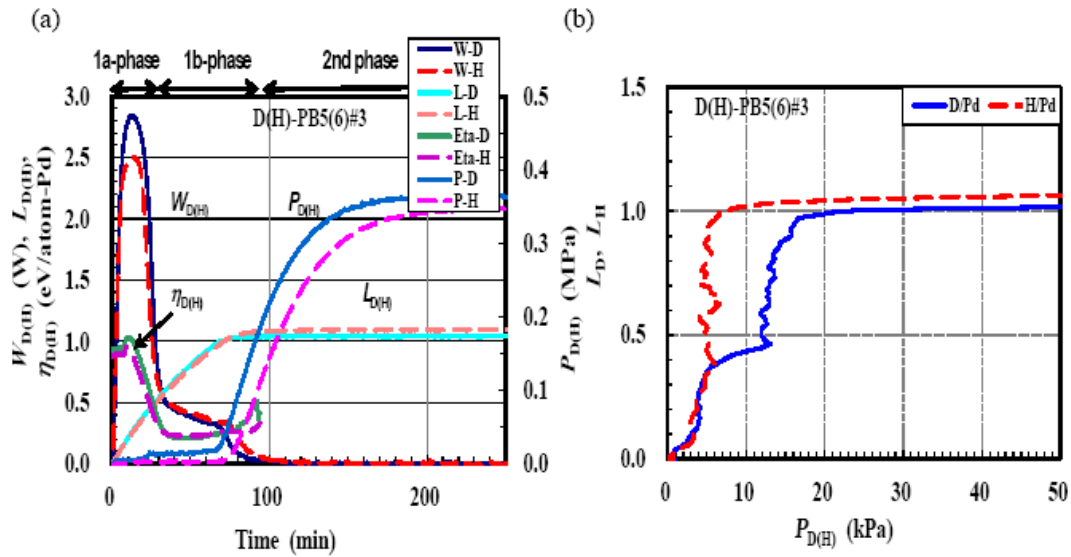
Figure 7. (a) Output power W(t) , pressure P(t) , time-resolved loading ratio L(t) and time-resolved specific sorption energy \eta(t) , (b) L(t) – P(t) diagram of the PB5(6)#3 runs.
