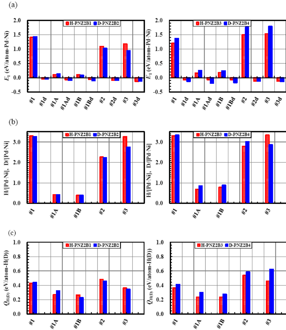
Figure 10. First-phase absorption parameters of the samples PNZ2B1 through PNZ2B4.
