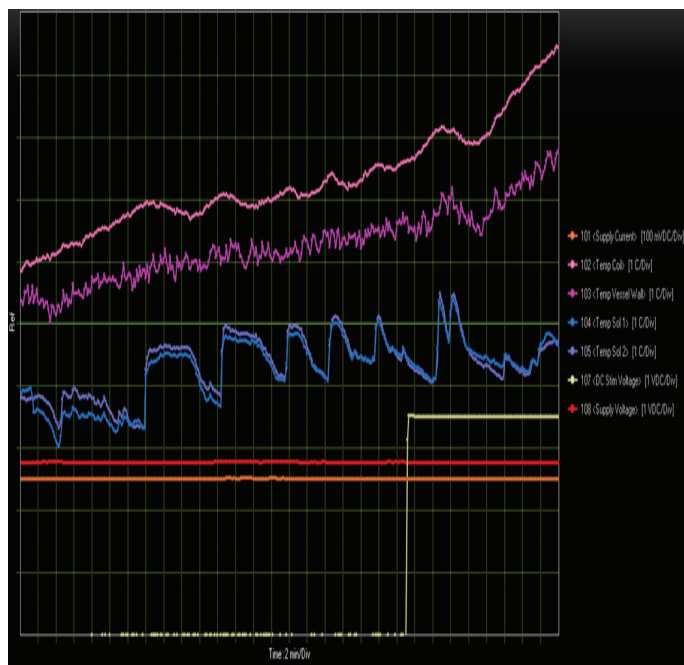
Figure 3. Experiment No. 3 data log showing temperature spikes. Experiment used Pd electrodes, anionic silica hydride, and lithium sulfate as an electrolyte in predominately heavy water.
