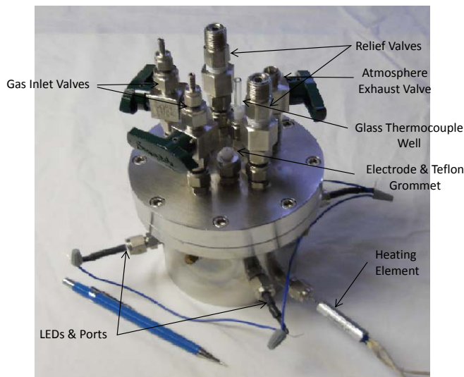
Figure 1. Reaction cell, showing LEDs and ports on the side. Electrodes and thermocouple wells can be seen on the top, along with relief valves and gas valves.
