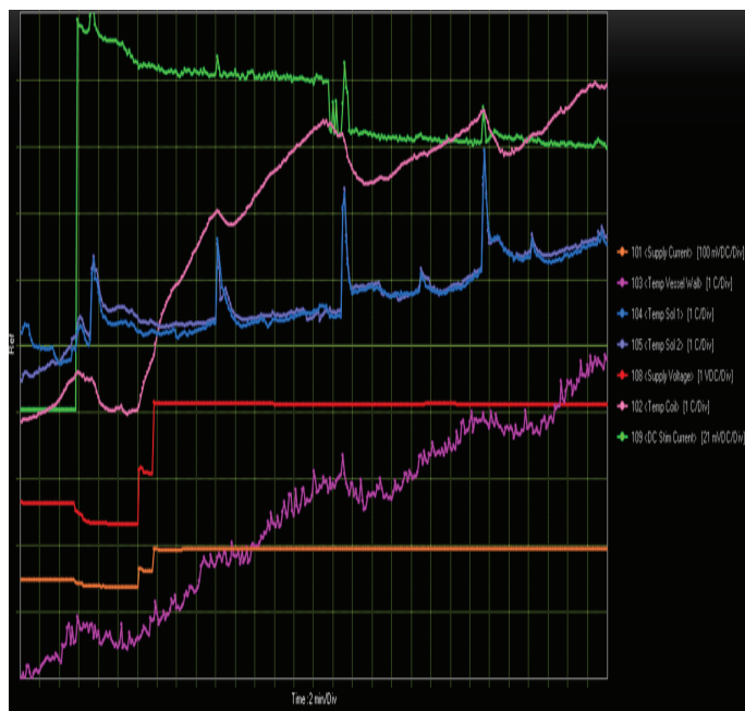
Figure 2. Experiment No. 1 data log showing temperature spikes. Experiment used Pd electrodes, anionic silica hydride, and lithium sulfate as an electrolyte in predominately heavy water.
