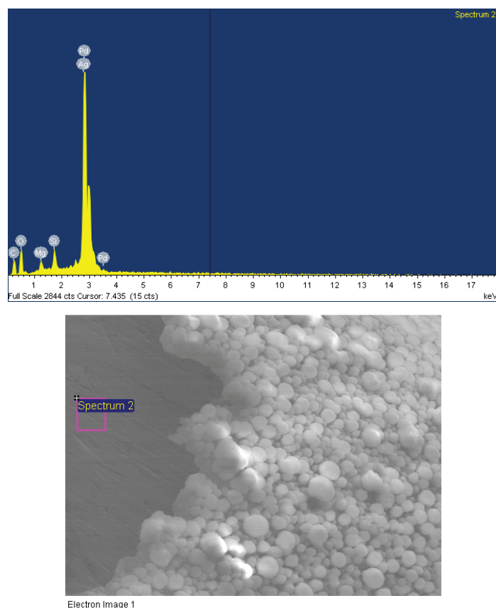
Figure 7. SEM photo of treated surface of a Pd electrode and accompanying EDS analysis showing the presence of Ag, a possible transmutation product of Pd.
