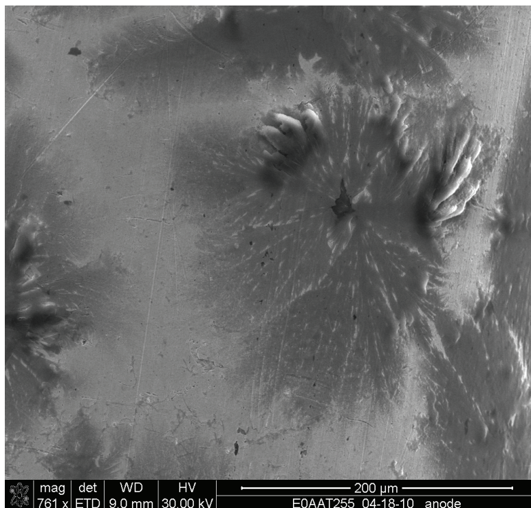
Figure 6. SEM photo showing a “volcanic site” on a gold electrode.
