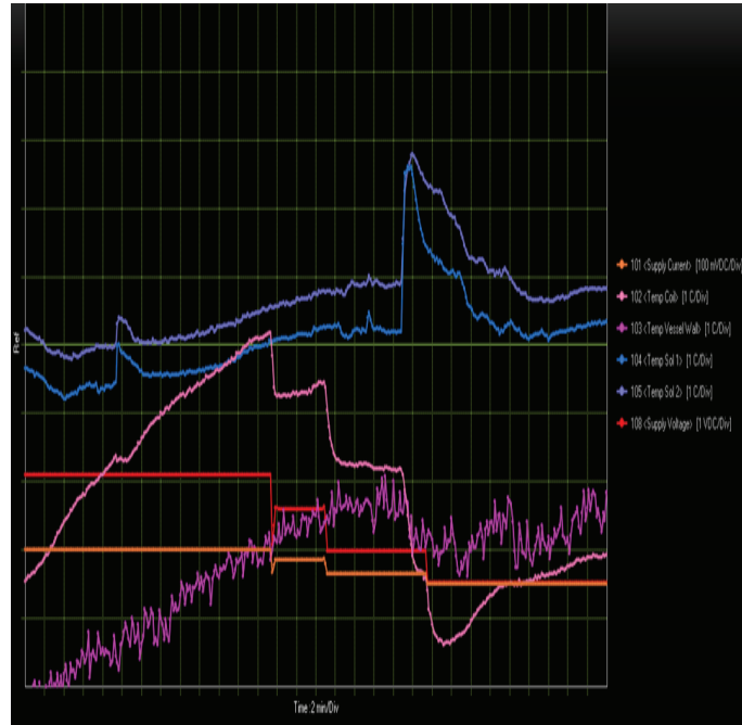
Figure 5. Experiment #3 used Pd electrodes, lithium metasilicate, and lithium sulfate as an electrolyte in predominately heavy water. Glass beads were strung onto the cathode.
