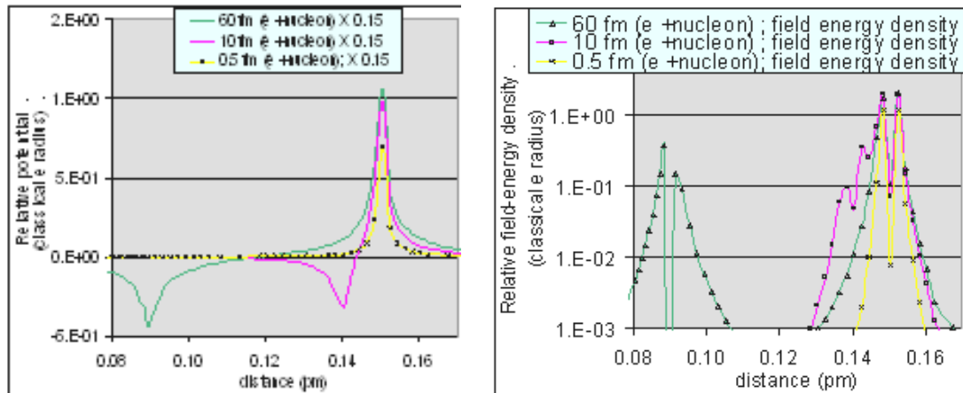
Figure 2. (a) Electric potential between, and (b) EM mass-energy distribution of, an electron (assuming a classical radius) and proton separated by 60, 10, and 0.5 fm. Note change in “size” of both particles, as they approach each other, and the change in vertical scale between (a) and (b).
