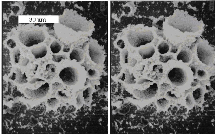
Figure 3. Stereo micrographs of complex craters, which were provided by Mizuno. They occurred on the surface of a gold cathode, which produced excess heat.
