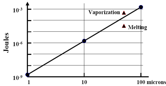
Figure 10. Plot of energies for cratering against crater diameter. The line is the extrapolation of the equation in Fig. 9. The two triangles give the energies for production of a 50 \mu\text{m} diameter crater by melting or vaporization, as given in Fig. 7.
