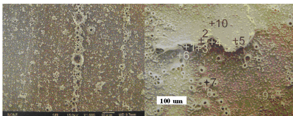
Figure 6. Craters approximately aligned with scratches on Pd cathodes. Left: These data are from Toriyabe et al. at ICCF-12. The crater density in this image is 1.6 \times 10^6 per \text{cm}^2 . Right: An image due to Zhang and Dash shown at ICCF-13. The crater density is 6.4 \times 10^4 per \text{cm}^2 . These images enable plotting of distributions (histograms) of crater diameters.
