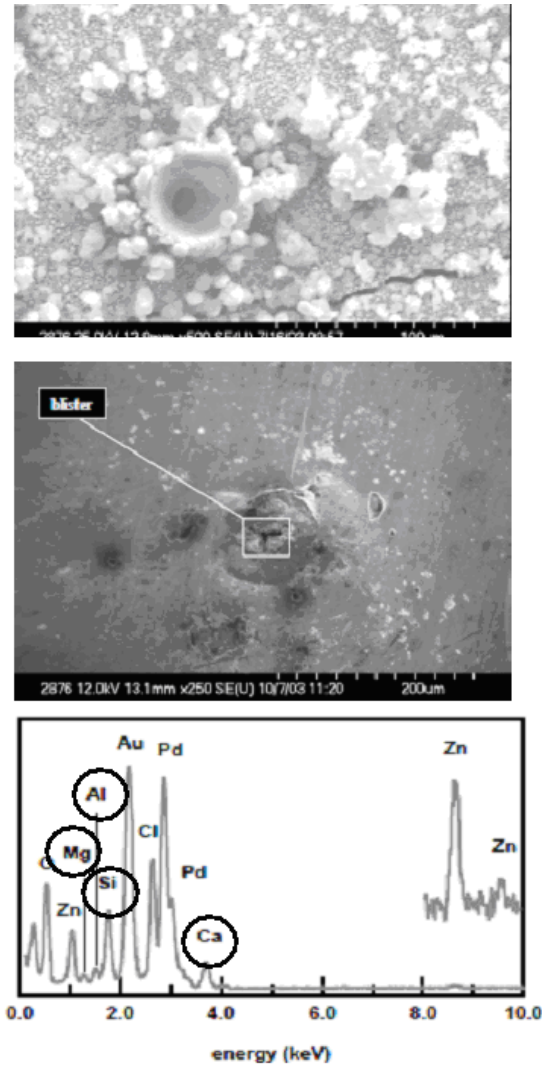
Figure 2. Micrographs showing a crater and a blister from the work of Szpak et al. The X-ray spectrum of elements near the blister is at the bottom. See the text regarding the elements within circles.
