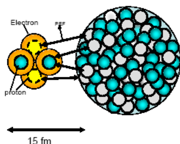
Figure 14. Image of strong interaction between 4H/TSC-minimum state and Ni nucleus.
