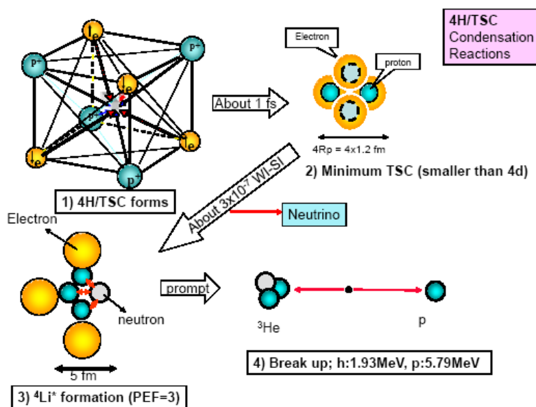
Figure 10. Illustration of 4H/TSC condensation motion and weak/strong fusion reaction [15].
