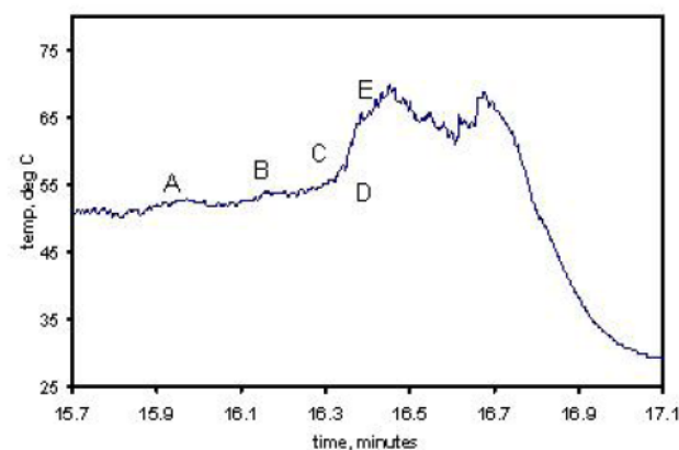
Figure 7. Temperature profile during thermal run-away
