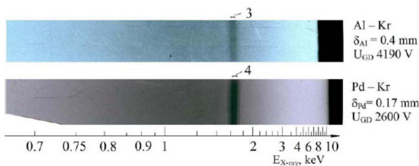
Figure 22. X-ray energy spectra in the band modes. 3,4 – energy is 1.65 keV, L 3 –M 1 transition for Kr.
