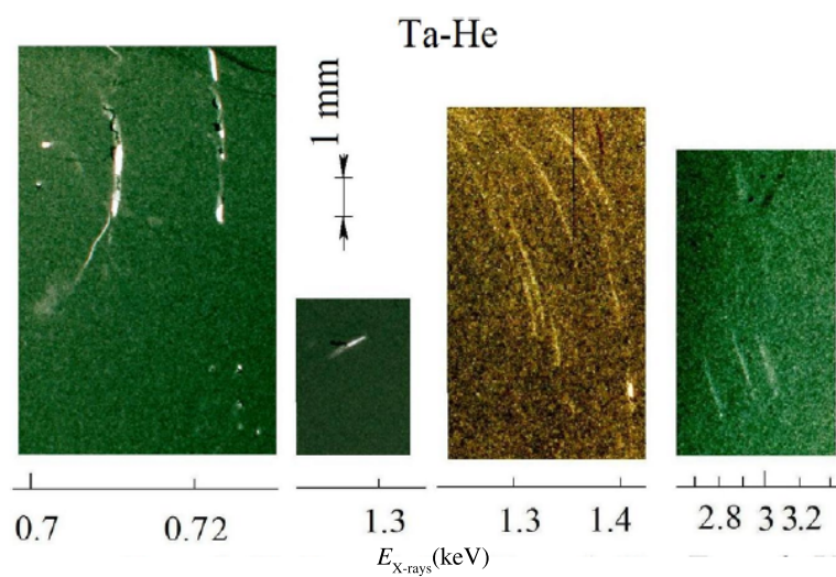
Figure 19. X-ray energy spectra in the spot modes for Ta cathode, He discharge.
