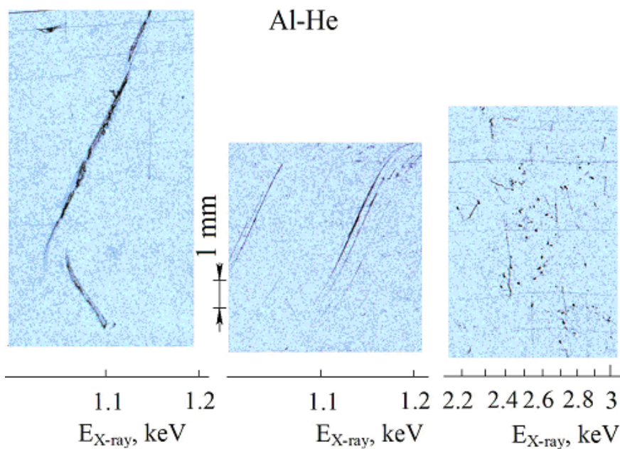
Figure 24. X-ray energy spectra in the spots and bands modes for Al cathode after the He glow discharge switch off. Exposition time is 20 h.
