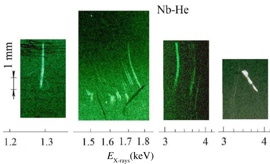
Figure 17. X-ray energy spectra in the spot modes for Nb cathode, He discharge.
