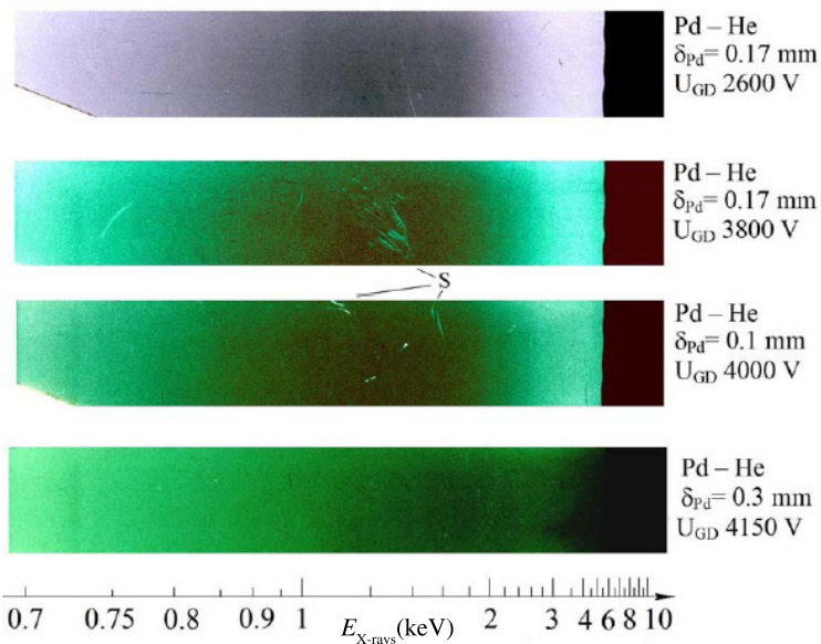
Figure 8. X-ray energy spectra from Pd cathode different thickness \delta_{Pd} . He discharge. U_{GD} is Glow Discharge voltage. S – white solarization spots of photoemulsion from X-ray monoenergetic beams with small angular divergence.
