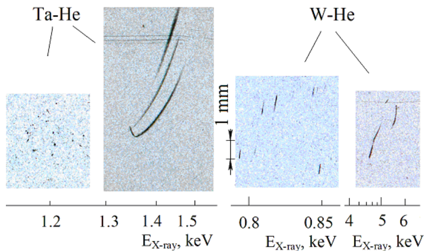
Figure 29. X-ray energy spectra in the spots and bands modes for Ta and W cathodes after the He glow discharge switch off. Exposition time is 20 h.
