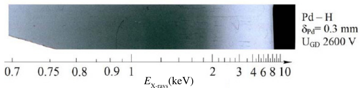
Figure 7. X-ray energy spectra from Pd cathode B H_2 discharge.
