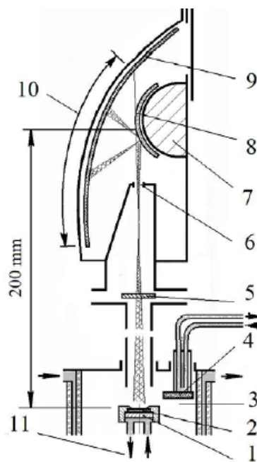
Figure 2. X-ray spectrometer 1–cathode holder, 2–cathode sample, 3–vacuum discharge chamber, 4–anode, 5–15 \mu\text{m} Be screen, 6–input slit of spectrometer, 7–crystals holder, 8–curved mica crystal, 9–X-ray film, 10–area of reflection spectra, 11–input and output cooling water.
