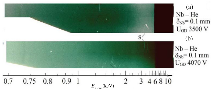
Figure 6. X-ray energy spectra from Nb cathode different thickness. He discharge. U_{GD} is Glow Discharge voltage. S – white solarization spots of photoemulsion from X-ray monoenergetic beams with small angular divergence.
