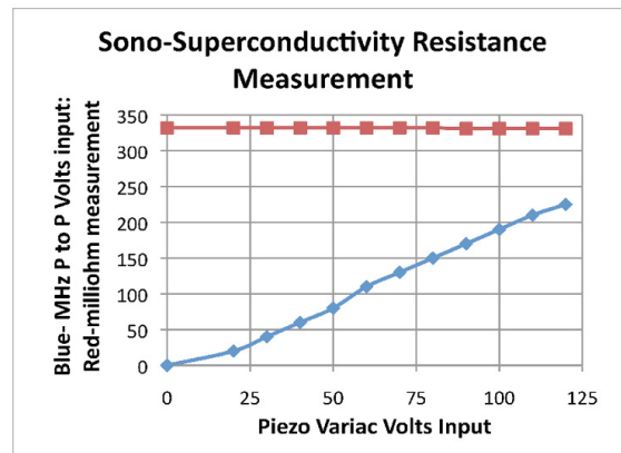
Figure 14. Reactor No. 2, superconductivity non-results.
