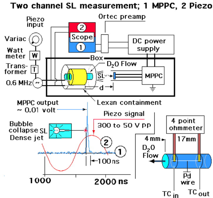
Figure 4. Reactor No. 2 superconductivity set-up with MPPC.
