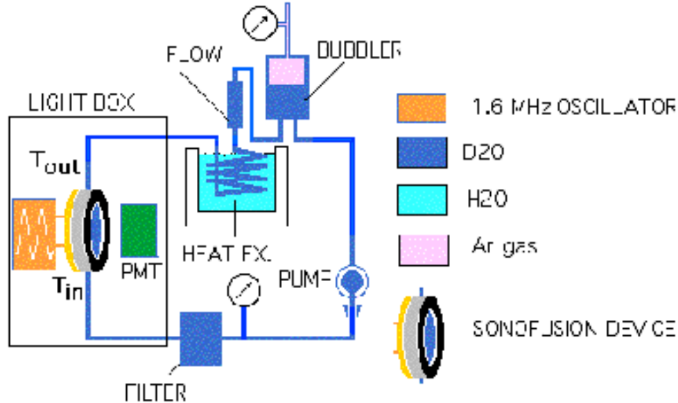
Figure 3. Reactor No. 1, sonofusion set-up.
