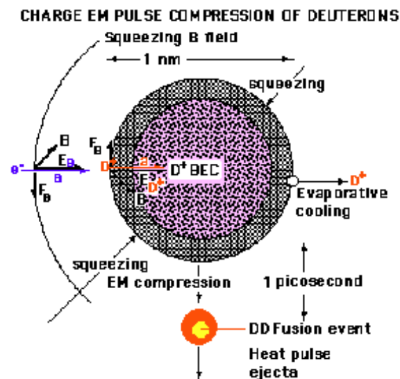
Figure 6. The cluster fusion of deuterons.
