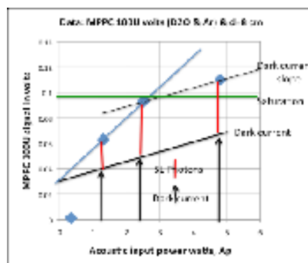
Figure 13. The MPPC photon measurement.
