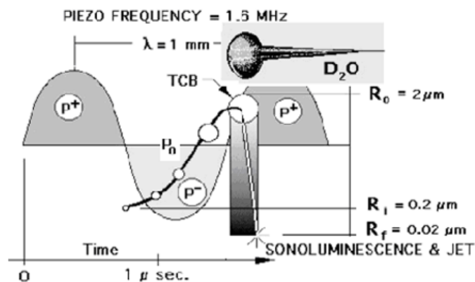
Figure 1. The 1.6 MHz TCB cycle .
