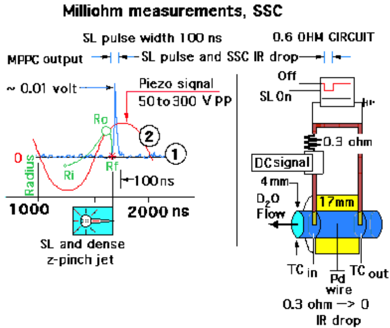
Figure 15. A piezo driven TCB collapse and the measurement of a Pd wire SSC.
