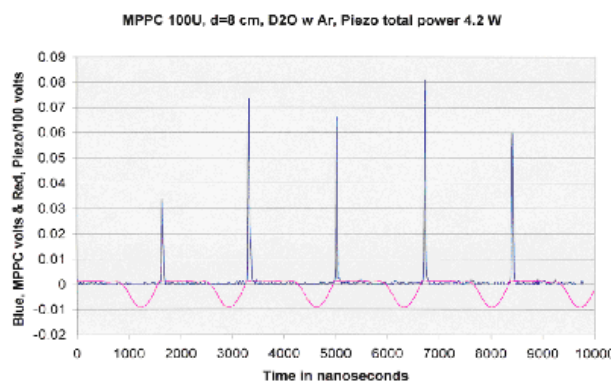
Figure 2. The MPPC SL pulse and MHz piezo volts.
