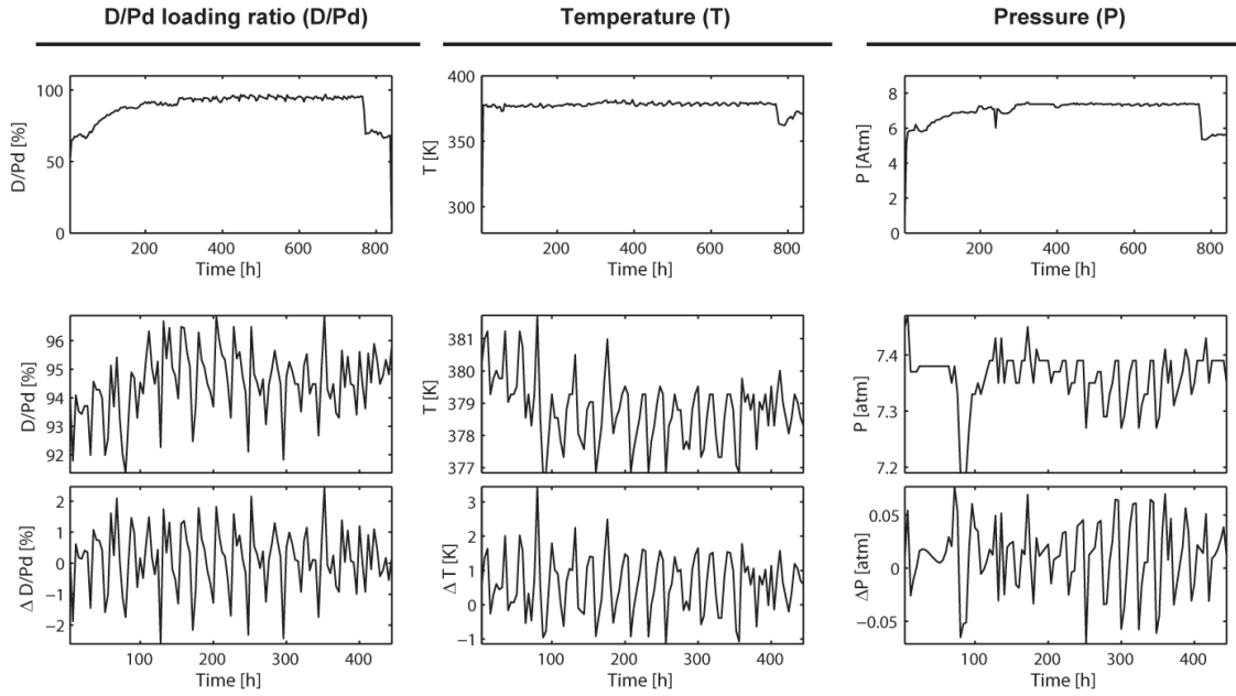
Figure 1. Raw signals (a–c), selected intervals (d–f) and results of the FIR-filtering (g–i).
