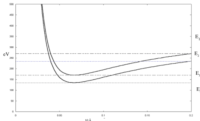
Figure 1. Features of V(r) and V(r) + W_{\max}/\sqrt{2} .
