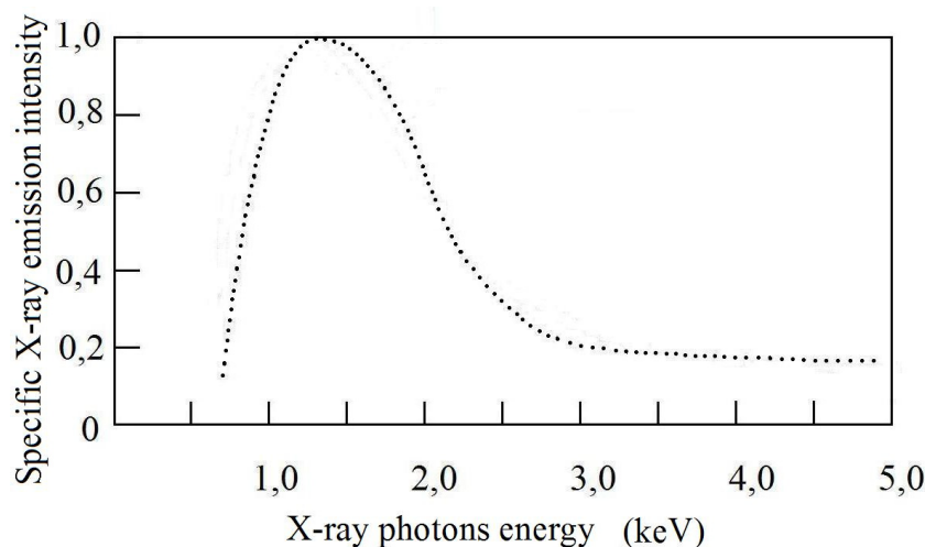
Figure 15. Continuum X-ray emission measured with the curved mica crystal spectrometer from a glow discharge experiment with a Pd cathode and D 2 gas.
