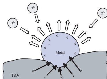
Figure 1. Cathodic protection.
