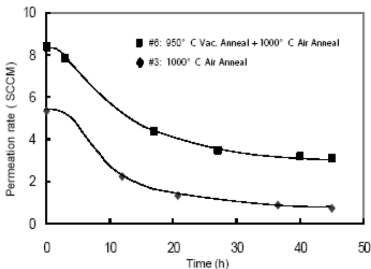
Figure 7. Comparison of the variations of permeation rate with time for samples Nos. 6 and 3.
