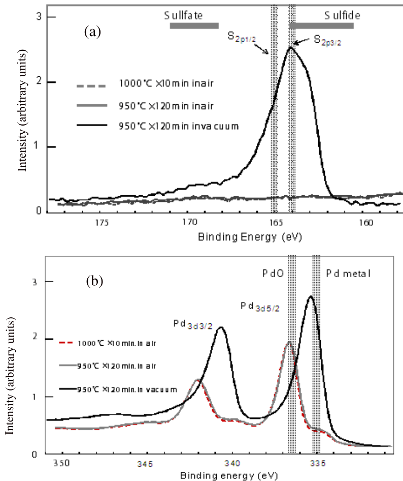
Figure 4. XPS spectra (a) around S 2p and (b) around Pd 3d for foil samples annealed in air (No. 3, No. 4) and in vacuum (No. 5).
