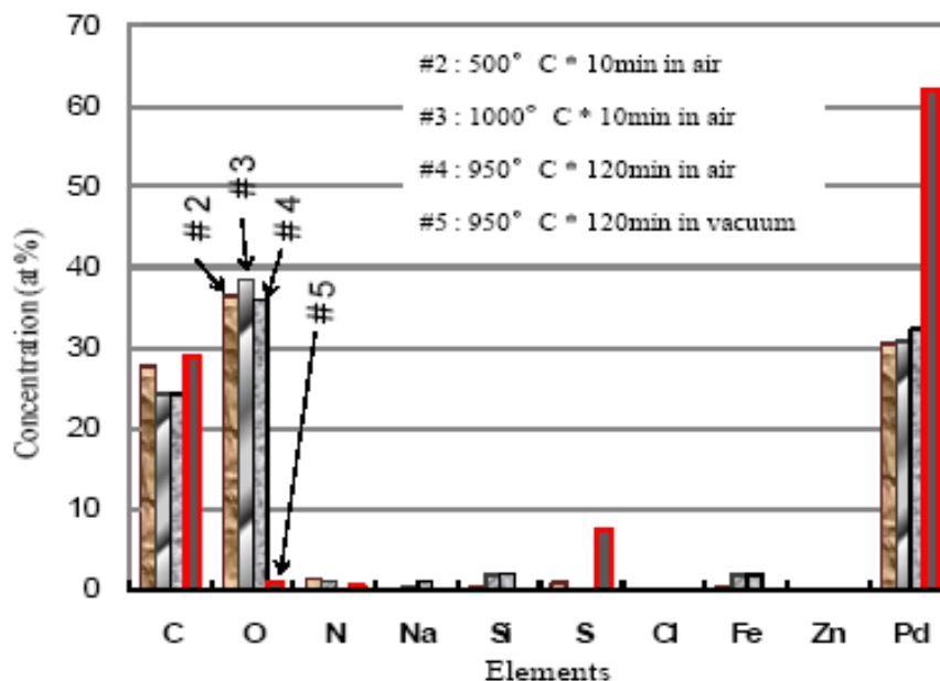
Figure 3. Elemental concentration on the surface layer of Pd after heat treatments.
