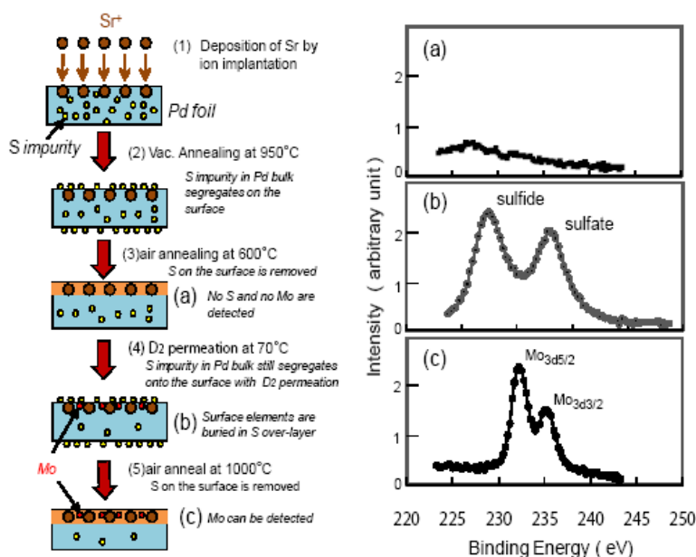
Figure 11. Schematics of the processes to detect Mo on the surface of Sr-ion implanted Pd after the deuterium permeation process, and XPS spectra around Mo 3d, (a) before D 2 permeation, (b) just after D 2 permeation treatment, (c) after adding an air-annealing at 1000°C to the D 2 permeated sample.
