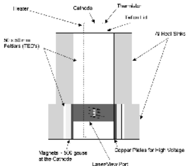
Figure 5. Schematic of the Seebeck calorimeter.
