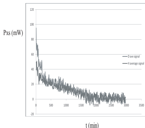
Figure 2. Excess power as a function of time for the Szpak experiment (courtesy of D. Cravens); comparison between heavy water cell result ( D_2O ) and light water control ( H_2O ). Pd was codeposited on polished copper in 0.3M LiCl in D_2O with 0.03 M PdCl_2 ; the current density used for codeposition was 1 mA/cm 2 for 8 hours, then 3 mA/cm 2 for 8 hours, then 5 mA/cm 2 for 8 hours.
