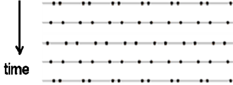
Figure 1. Longitudinal optical modes where adjacent lattice atoms/ions move in opposite directions along a common axis.
