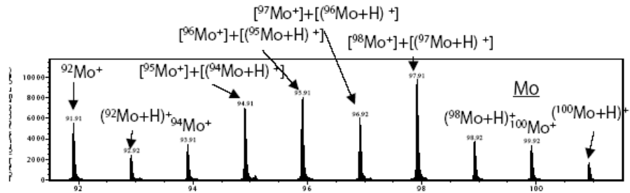
Figure 5. TOF-SIMS spectrum of the surface of Mo metal plate, and assignment of each peak.
