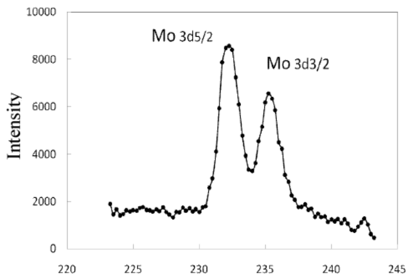
Figure 2. XPS spectrum around \text{Mo}_{3d} for ^{88}\text{Sr}^+ implanted Pd/CaO multilayer sample after \text{D}_2 permeation followed by annealing in the air.
