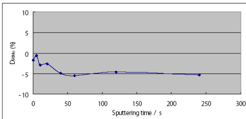
Figure 6. Relationship between deviations of measured intensities from theoretical intensity for ^{96}\text{Mo}^+ calculated with Eq. (3) and sputtering time.
