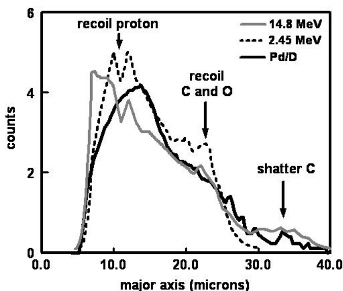
Figure 4. Track size distribution for CR-39 detectors that have been exposed to 2.45 and 14.8 MeV neutrons are overlaid with the track size distribution obtained on the backside of a CR-39 detector used in a Pd/D co-deposition experiment.
