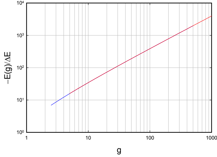
Figure 1. Self-energy as a function of the dimensionless coupling strength g for \Delta n = 91 (blue) and \Delta n = 151 (red).
