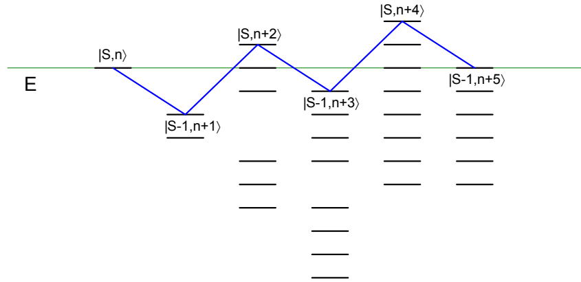
Figure 3. Levels and transitions for lowest loss pathway in perturbation theory starting from |S, S, n\rangle = |S, n\rangle , in the case of \Delta E = 5\hbar\omega_0 .
