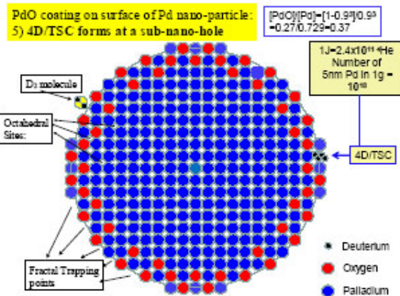
Figure 8. Eventual 4D/TSC fusion on surface.
