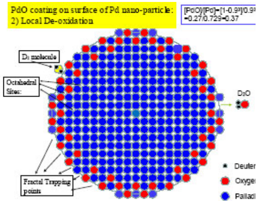
Figure 5. D 2 O molecule going out.
