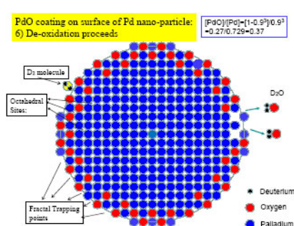
Figure 13. Extended sub-nano dips by D 2 O formation.
