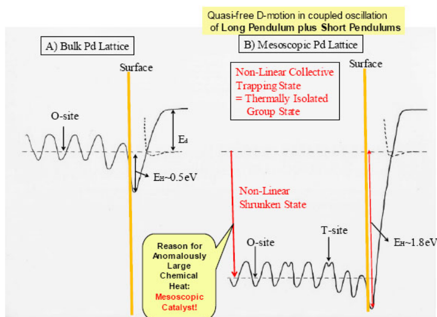
Figure 18. Collective shrunk state potential of Pd nano-particle for D(H) trapping, right figure, compared with a bulk metal trapping potential, left figure.
