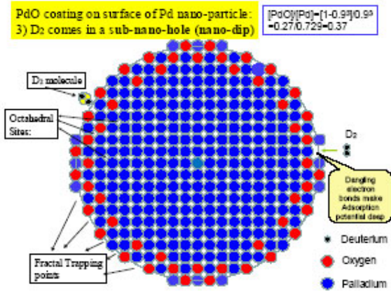
Figure 6. SNH traps D 2 incoming.
