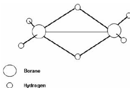
Figure 3. The configuration of atoms in diborane, B_2H_6 [6, 7].
