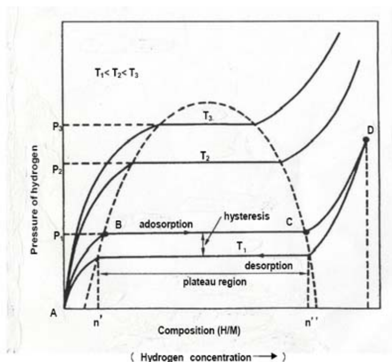
Figure 1. Pressure-composition isotherm adsorption with the parameter, temperature [4].
