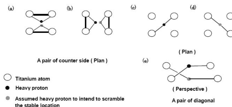
Figure 7. The heavy protons model in the O-site. (a), (b): a pair of counter side (plan), and (c), (d): a pair of diagonal side (plan), (e): a pair of diagonal side (perspective).
