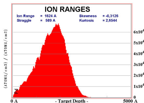
Figure 1. Boron ion distribution vs. target depth.
