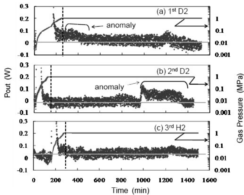
Figure 10. The same data as in Fig. 8 are displayed with the vertical axis enlarged by 10-fold. The vertical dotted lines indicate the boundary of the first stage and the second stage, and the horizontal gray lines the zero level of P_{\text{out}} .
