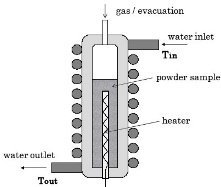
Figure 1. Schematic of the calorimeter.
