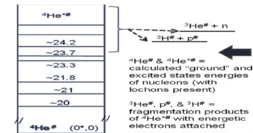
Figure 4. Energy levels and possible decay branches associated with the lochon model D + D to {}^4\text{He}^{*#} fusion reactions and minimum D + D input energy levels of {}^4\text{He}^{\#} . Note that these values include the tightly bound-electron-induced adjustments to the nuclear potential and the mass energy of the atomic and shrunken-orbit electrons.
